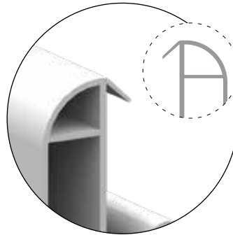
Insulation flap (sealing to water coextrusion)
